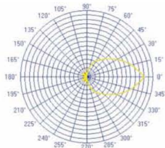
Single Emitter Polar Plot @ 1kHz
